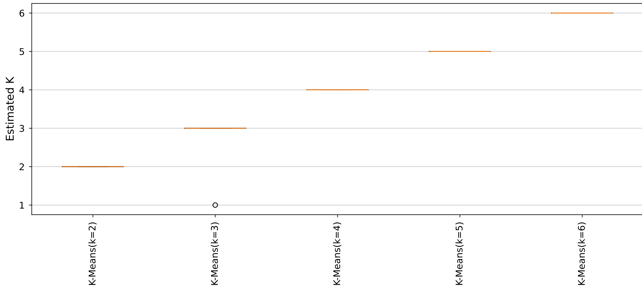
YARA Rules Estimated K Distribution (Cluster31_Size6 dataset)
